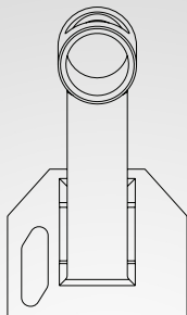
4.8" x 20.5" Boxed Channel Single CNC Deck Exclusive Rail Connector NECO Integrated Sealed Headset Threadless IHC System Anodised Gold Finish
